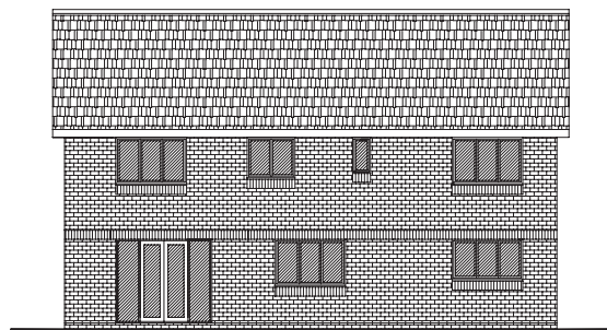
REAR ELEVATION
