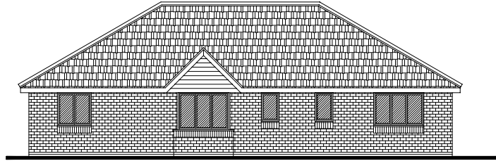
REAR ELEVATION
