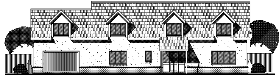
FRONT ELEVATION
