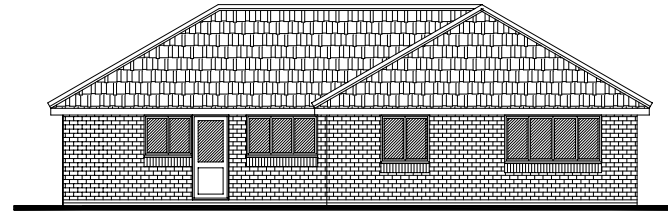
REAR ELEVATION
