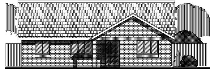
FRONT ELEVATION
