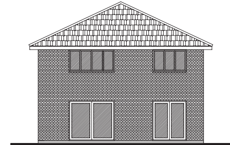
REAR ELEVATION
